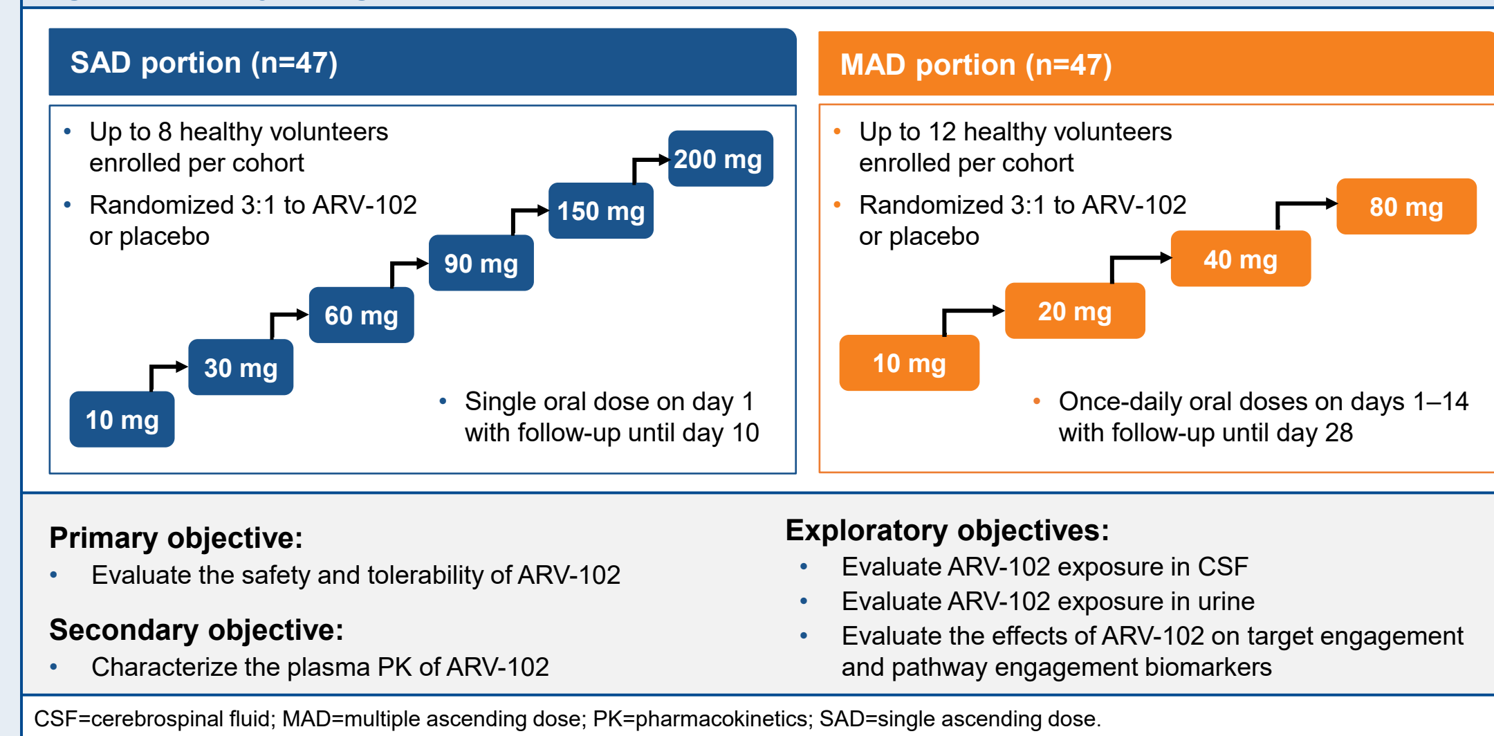
Figure 2: Study design
